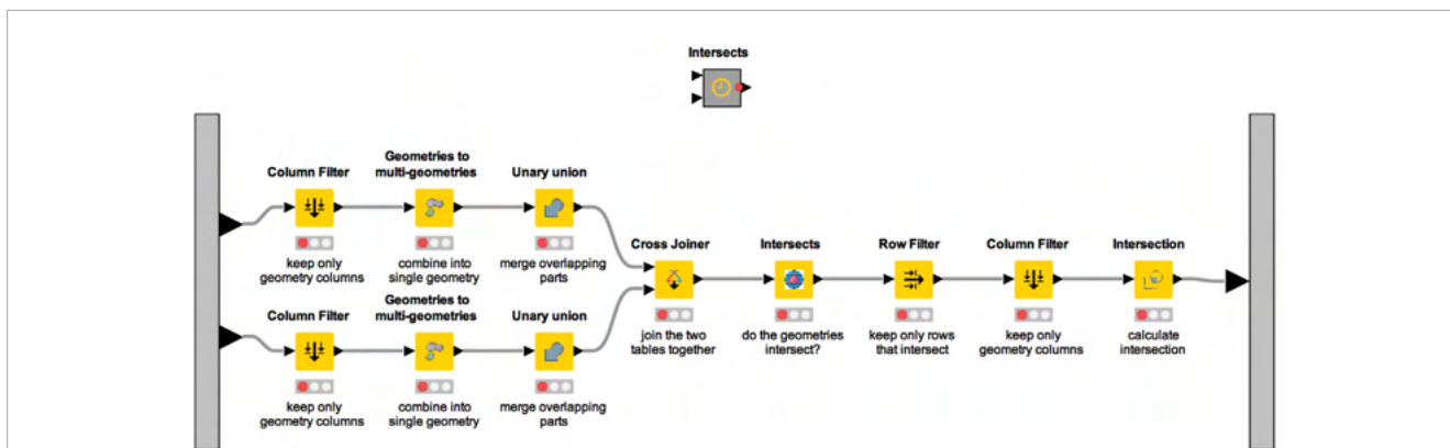
FIGURE 4 Example of an Intersects workflow metanode. This metanode takes in two tables and removes their non-spatial columns before collapsing the geometry into a single row. The two tables are then joined, and checked to see if they intersect before the intersection operation is performed. A single data table with intersected geometry is then output.
